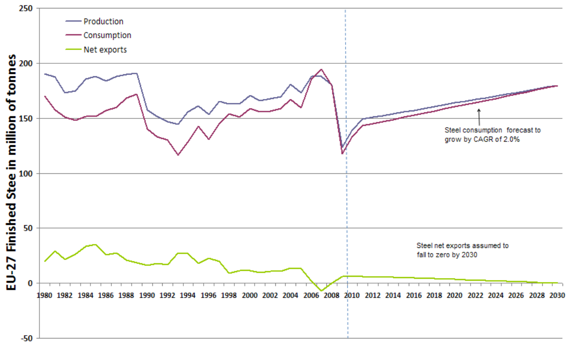
Figure 9: Iron & Steel production, demand and net export for EU27 up to 2030
